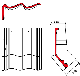
knikgevelpan links 140°
