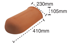
Ridge Hip / End
