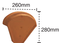
Ridge End Cap
