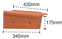
Right Verge Tile (2.9pcs/metre)
