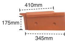
Left Verge Tile (2.9pcs/metre)
